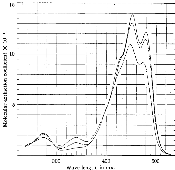
Fig. 2.—Molecular extinction curves of \beta -carotene in hexane: — fresh solution of the all- trans compound, --- mixture of stereoisomers after refluxing, and -·-· after iodine catalysis.
