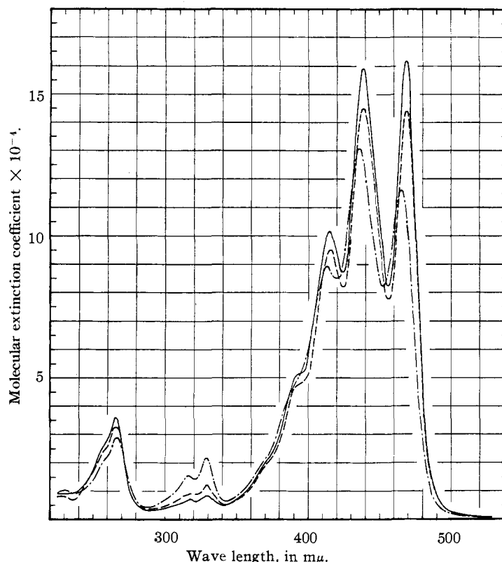
Fig. 6.—Molecular extinction curves of 5,6-dihydro- \alpha -carotene in hexane: — fresh solution of the all- trans compound, --- mixture of stereoisomers after refluxing, and - - - after iodine catalysis.
