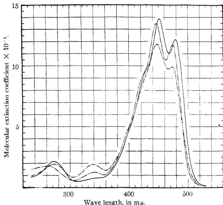
Fig. 3.—Molecular extinction curves of neo- \beta -carotene U, compared with that of \beta -carotene in hexane: — \beta -carotene, - - - fresh solution of neo- \beta -carotene U, and ···· mixture of stereoisomers obtained from neo U by iodine catalysis.
