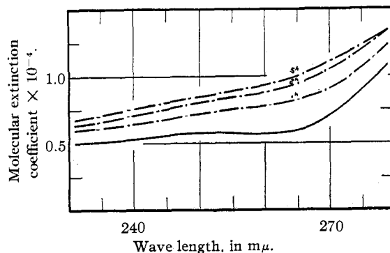
Fig. 8.—Molecular extinction coefficients of vitamin A in hexane between 230 m\mu and 280 m\mu : — fresh solution of crystalline vitamin A (the readings were concluded within 21 min. after dissolution), --- one, two and five hours after the addition of iodine (the five-hour curve remained practically unaltered after seven hours).
