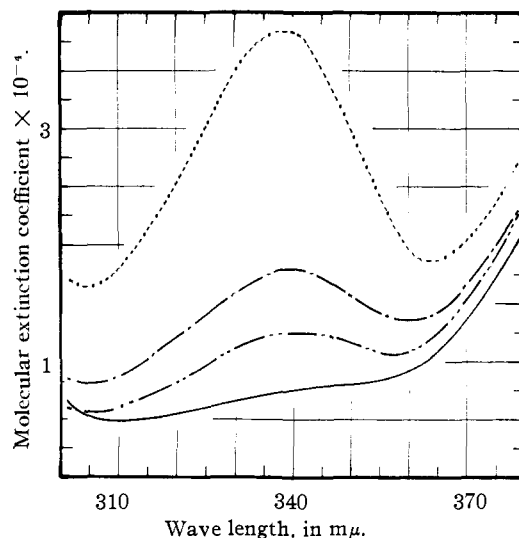
Fig. 4.—Molecular extinction curves of some \beta -carotene stereoisomers in the cis -peak region (in hexane): — all- trans - \beta -carotene, - - - neo U, ···· mixture of isomers adsorbed below the all- trans form, and — · — · iodine equilibrium mixture.
