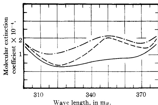
Fig. 5.—Molecular extinction curves of \beta -carotene in chloroform: — fresh solution of the all- trans compound, --- after iodine catalysis, and - - - the corresponding section of the curve published by Gillam, et al. 15 for butter carotene.
