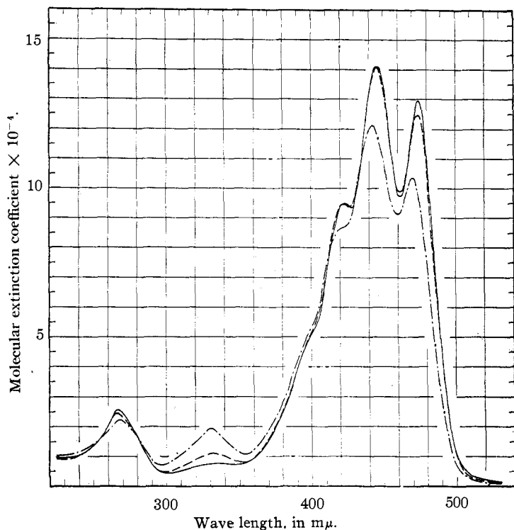
Fig. 7.—Molecular extinction curves of 5,6-dihydro- \beta -carotene in hexane: — fresh solution of the all- trans compound, --- mixture of stereoisomers after refluxing, and - - - after iodine catalysis.
