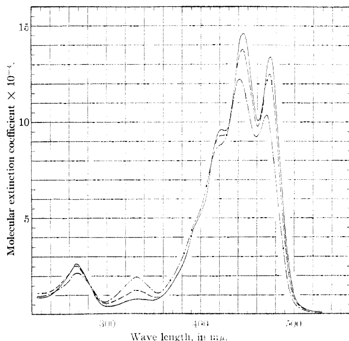
Fig. 1.—Molecular extinction curves of \alpha -carotene in hexane: ——— fresh solution of the all- trans compound, - - - mixture of stereoisomers after refluxing, and - · - after iodine catalysis.
